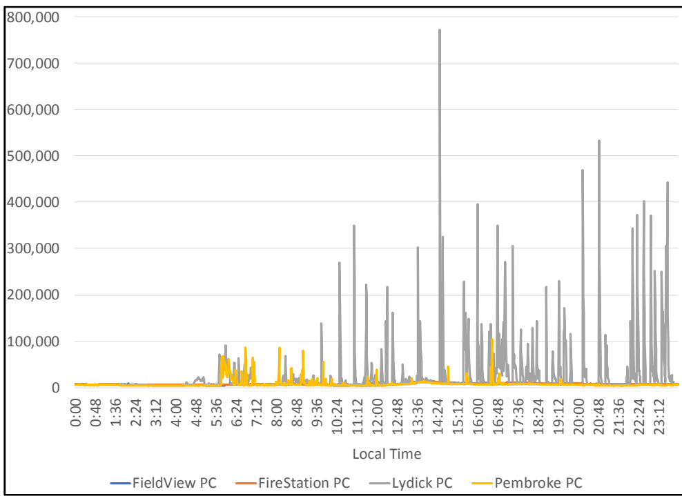
Figure 20: Particle Count, Lydick Site, Downwind of Airport, Runway 23 in Use, February 28, 2016
