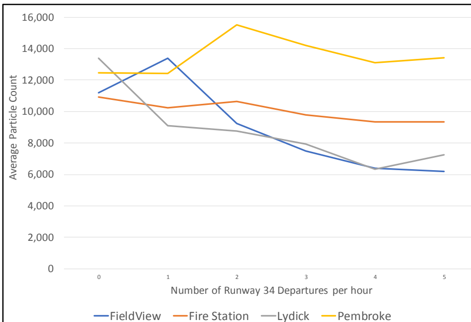
Figure 24: Impact of Runway 34 Departures on Particle Count Levels, 2016
