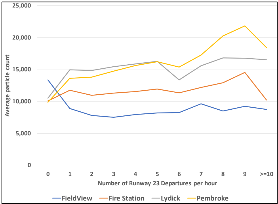
Figure 19: Impact of Runway 23 Departures on Particle Count Levels, 2016
