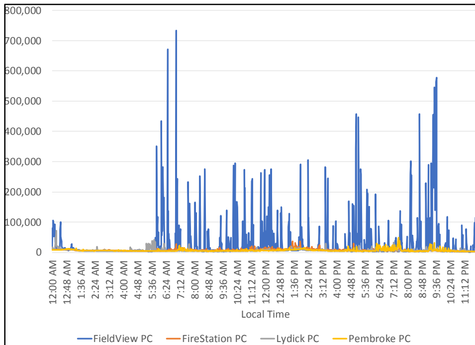
Figure 12: Particle Count At Field View Site, Downwind of Airport, March 14, 2016
