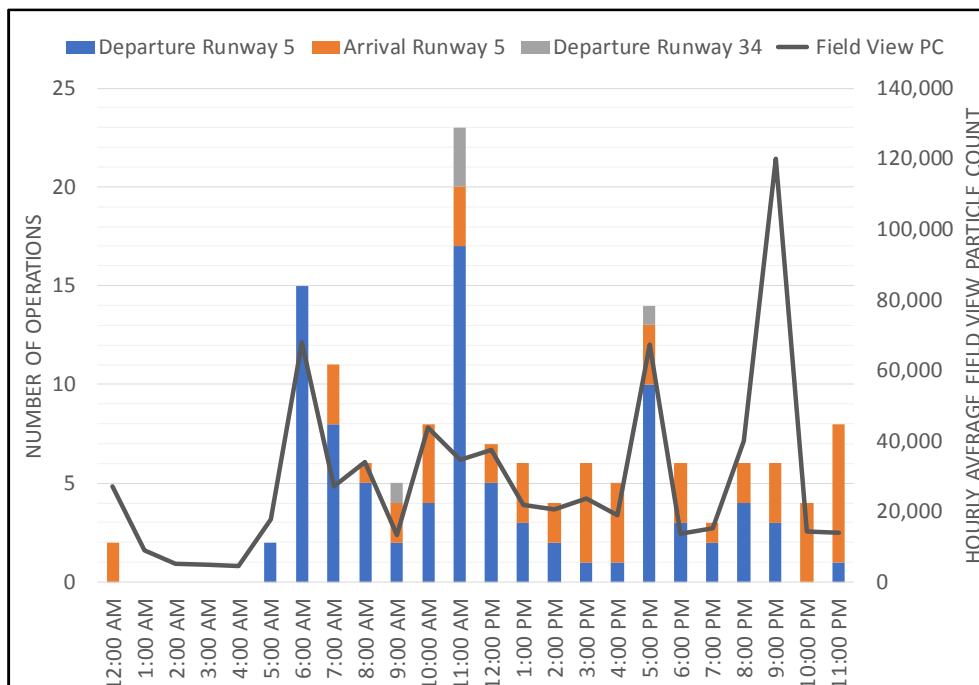
Figure 13: Hourly Operations Versus Field View Particle Count, March 14, 2016
