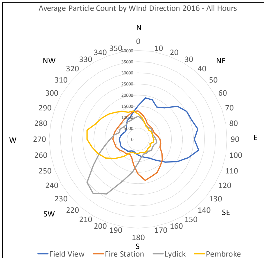
Figure 7: Effect of Wind Direction on Particle Count, 2016
