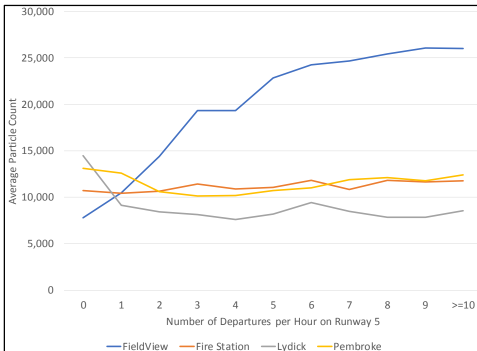
Figure 11: Impact of Runway Departures on Particle Count Levels, 2016
