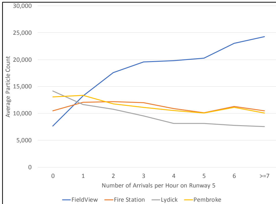
Figure 10: Impact of Runway 5 Arrivals on Particle Count Levels, 2016
