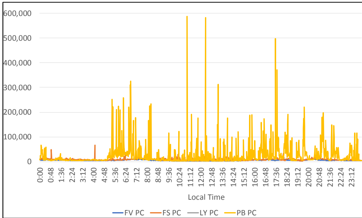
Figure 26: Particle Count, Pembroke Site, Downwind of Airport, Runways 23 and 34 in Use, December 2, 2016
