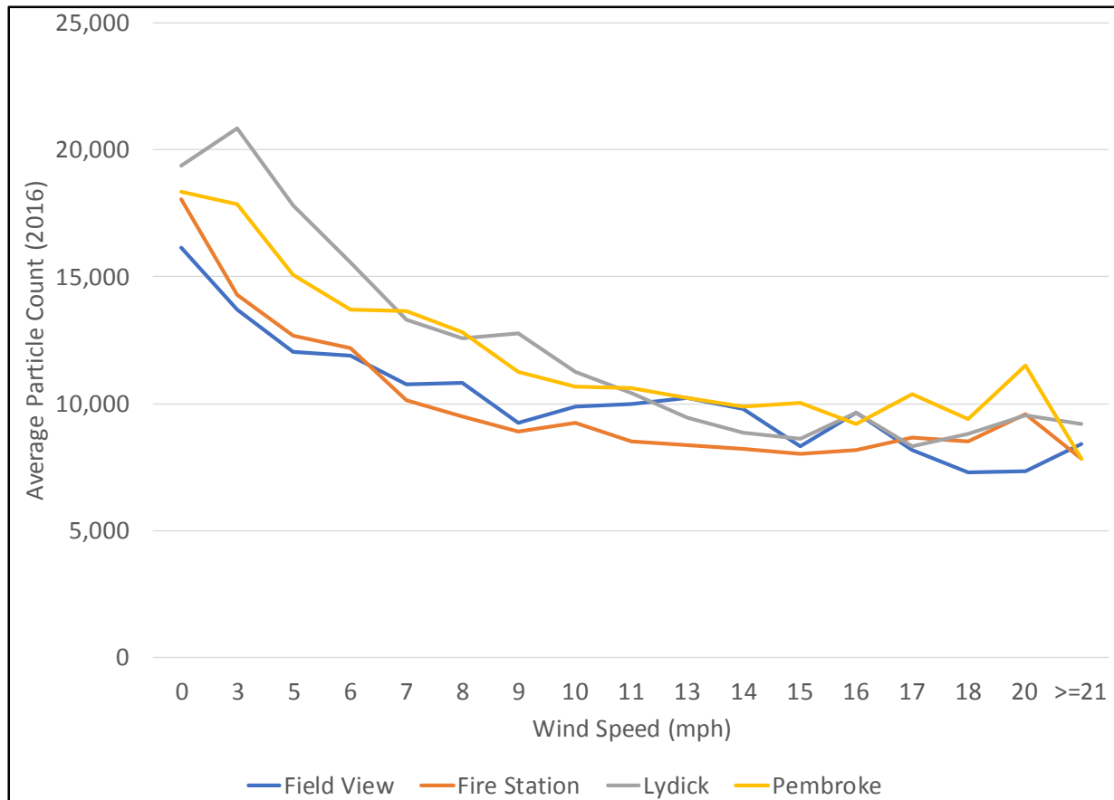
Figure 6: Effect of Wind Speed on Particle Count (Ultra-Fine Particle Concentration), 2016
